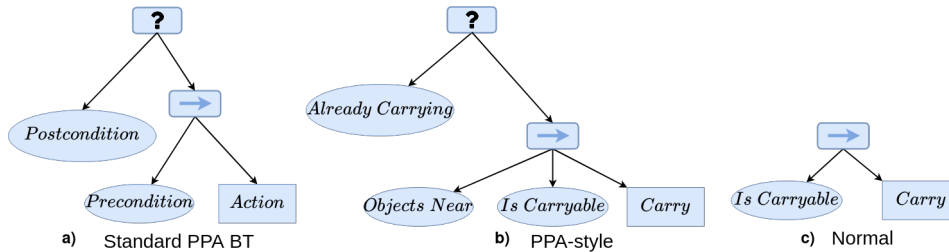
Figure 1: BTs for primitive behaviors. a) General PPA-style BT. CompositeSingleCarry primitive behavior represented with b) PPA-style and c) nominal trees.
