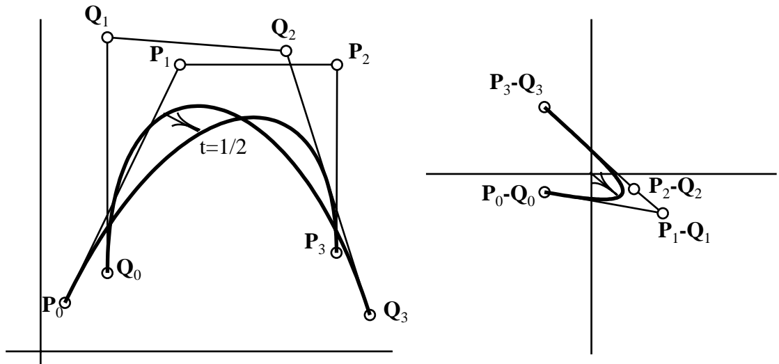
Figure 2.11: Difference curve.
