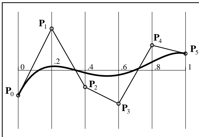
Figure 2.19: Explicit Bézier curve
