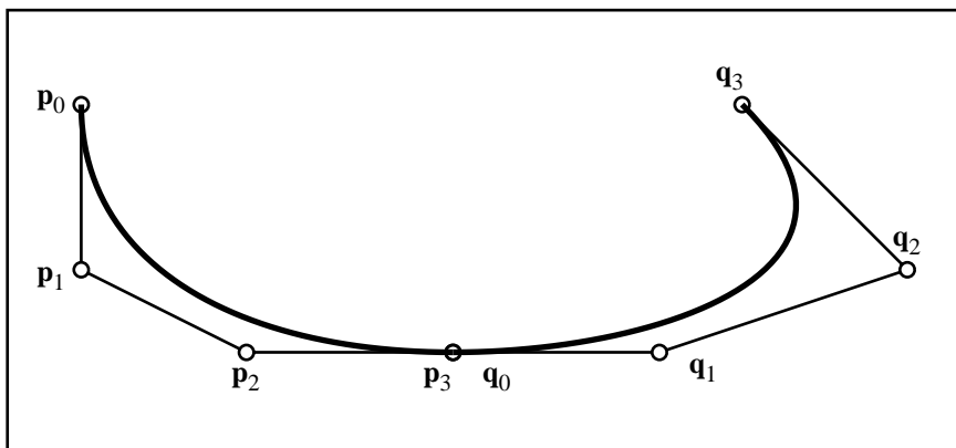
Figure 2.13: C^2 Bézier curves.
