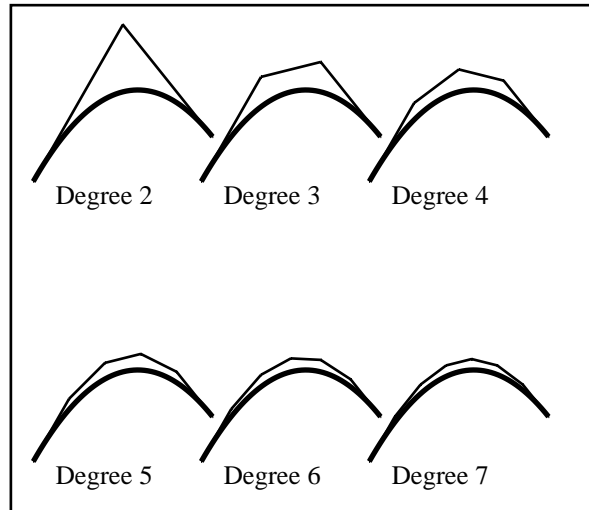
Figure 2.10: Repeated degree elevation.
