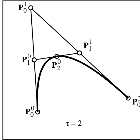
Figure 2.8: Subdividing a quadratic Bézier curve.
