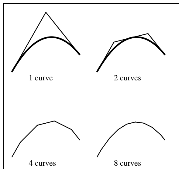
Figure 2.7: Recursively subdividing a quadratic Bézier curve.
