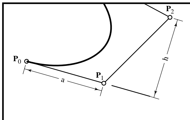
Figure 2.14: Endpoint curvature.
