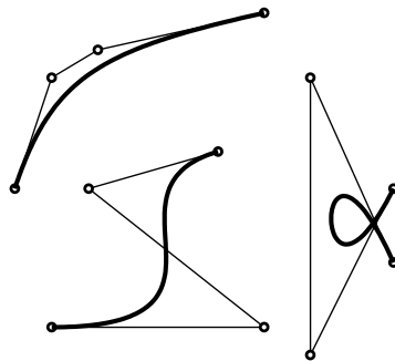
Figure 2.4: Examples of cubic Bézier curves
