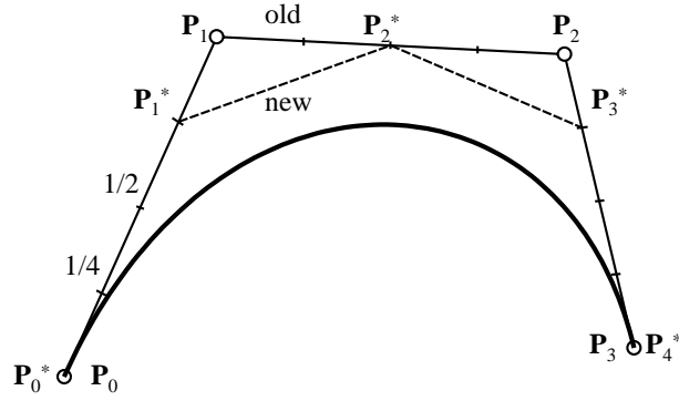
Figure 2.9: Degree elevation.
