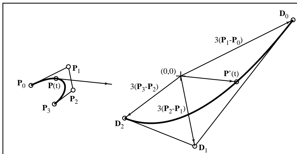
Figure 2.12: Hodograph.
