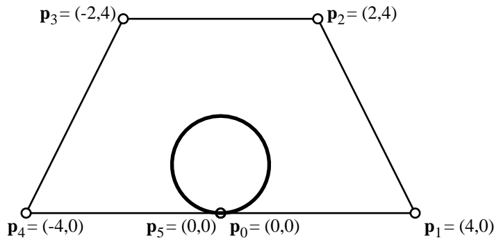
Figure 2.18: Circle as Degree 5 Rational Bézier Curve
