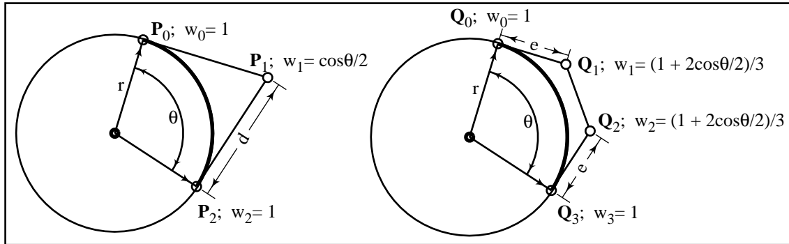
Figure 2.17: Circular arcs
